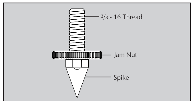
Figure 5. The ETC™ Spike.
